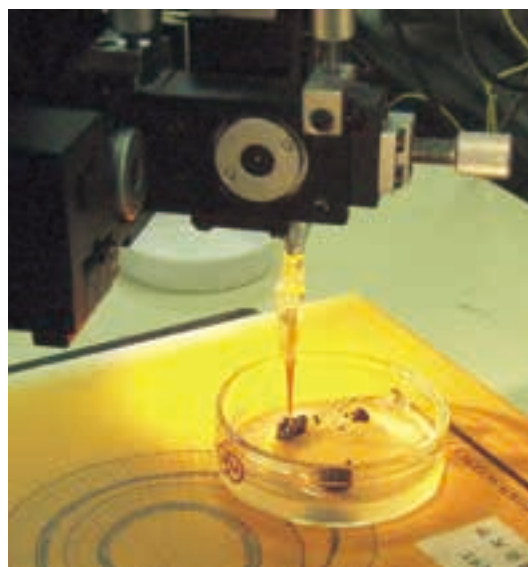
土壌団粒中の酸素濃度変化を10μm 刻みで測定 Microprofiling of oxygen gas concentration in the tiny soil aggregate
