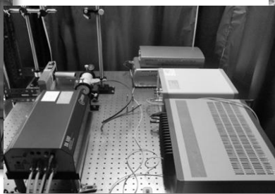
Laser Induced Fluorescence
