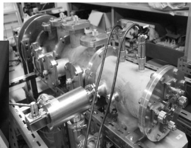
Small Helicon Device
