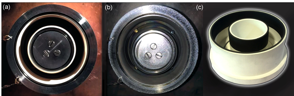
FIG. 10. A comparison of the MaSMi-60's discharge channel and pole faces before (a) and after \sim 20 h of operation (b). Note the uniform layer of carbon deposited on the inner and outer channel walls, suggesting the presence of magnetic shielding, and the level of front inner and outer pole face erosion. Reprinted with permission from Conversano et al. , Paper IEPC-2015-100. Copyright 2015 EPRS. 63 (c) Conducting discharge channel walls with the graphite inserts for testing the magnetic shielding operational regimes. Reprinted with permission from J. Appl. Phys. 122, 033305 (2017). Copyright 2017 AIP Publishing LLC. 70
