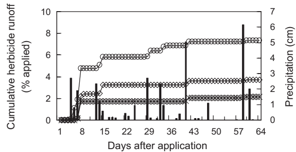
Fig. 10. Simulated runoff losses of herbicide mefenacet by different excess water storage depth (EWSd) management 35 —: Precipitation, —*—: EWSd = 2 cm, —◇—: EWSd = 1 cm, —○—: EWSd = 0 cm.
