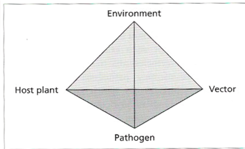
Fig. 3.11 The disease tetrahedron.
