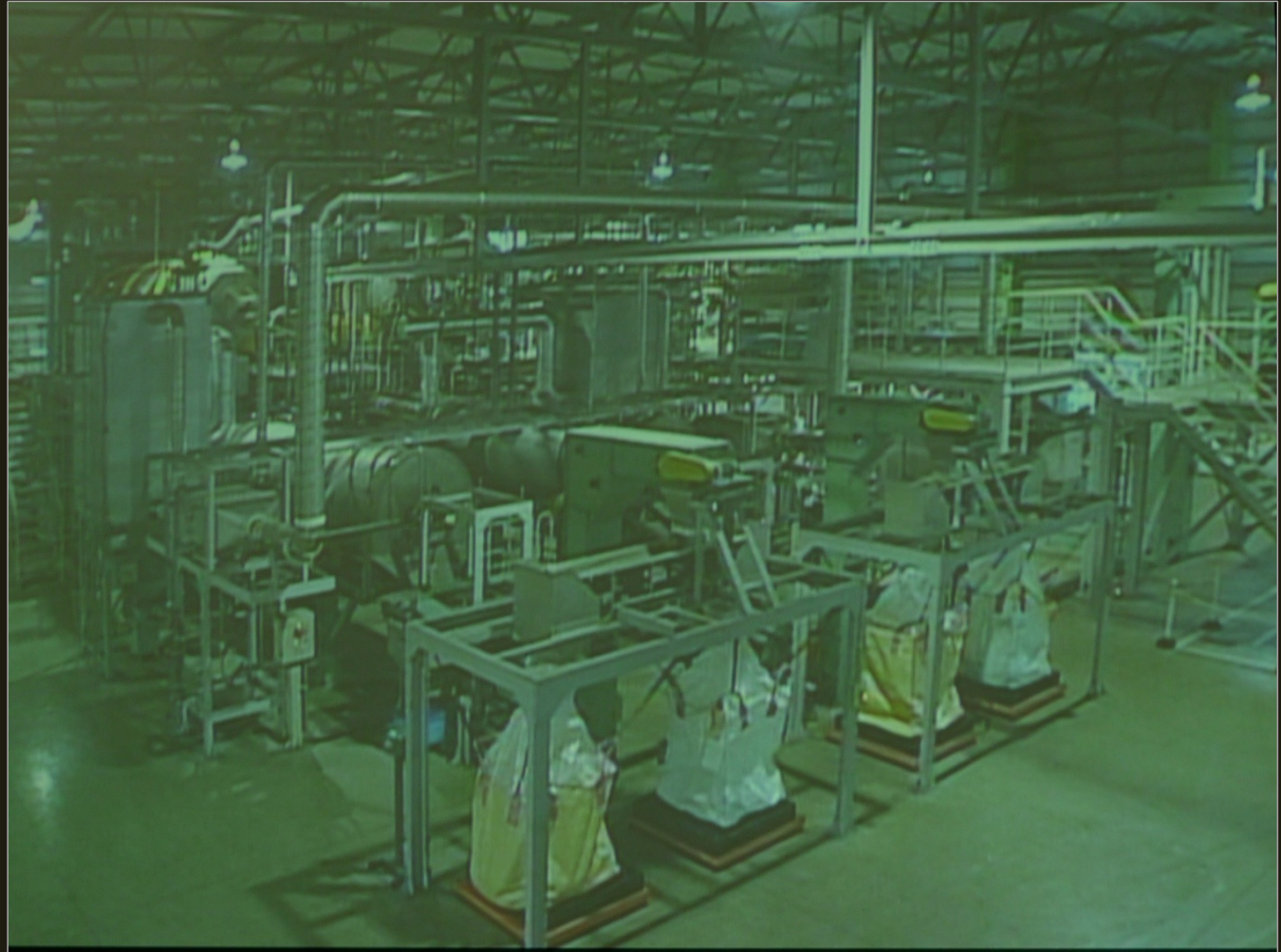
fluorescent material stripping machine
